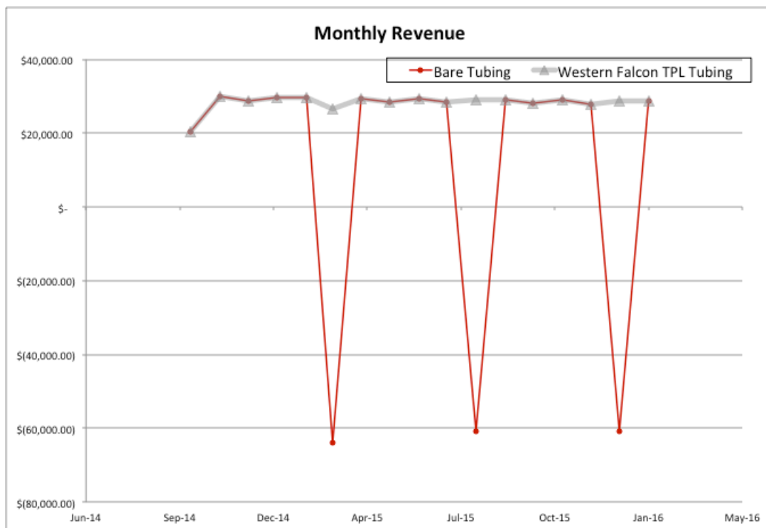
Figure 10 – Comparative Monthly Single Well Revenue Before and After Installation of TPL Tubing For Case Study Four
